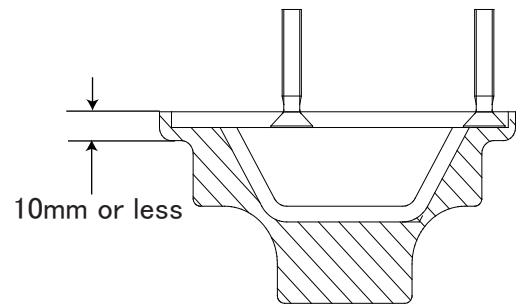
< Cross section of Engine bolt >
